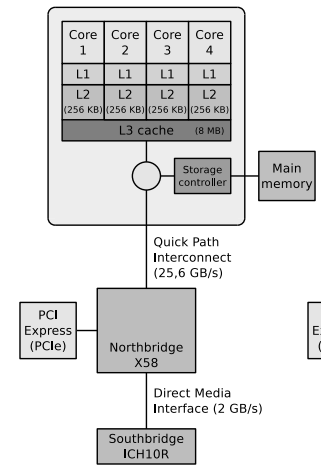
Intel Core i7-965 Extreme Edition
